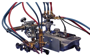
SP-300 Torch Set ■ 2 torch unit with mechanical automatic torch height control ■ Maintains angle of 2 torches for accurate Y and X bevel cuts
