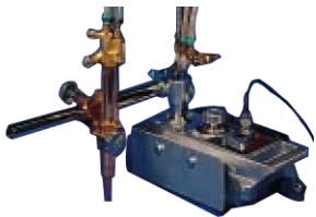
L-100 Torch Set ■ Heavy duty torch designed to cut up to 300 mm plate thickness. ■ Water cooled
