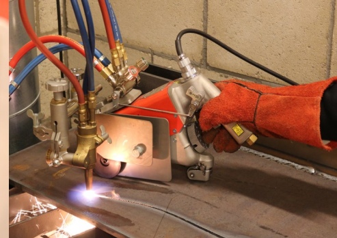
Hand guided cutting
